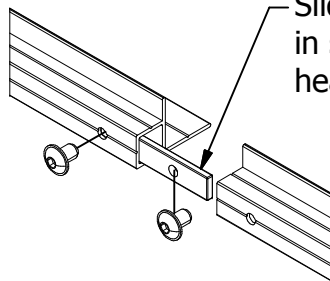
Ceiling Guide Track Splice
