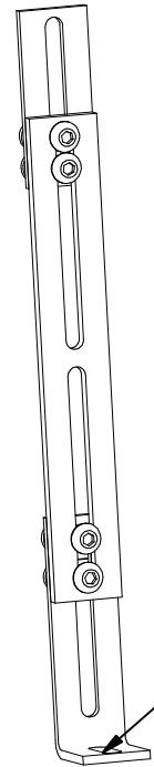
Adjustable Support Bracket
